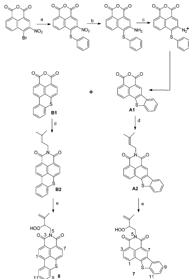
Scheme 2. The synthetic route of heterocyclic-fused naphthalimides: (a) PhSH, EtOH, reflux, 4 h, 51% yield; (b) \text{SnCl}_2/\text{HCl} , 92.6% yield; (c) Pschorr cyclization; (1) \text{NaNO}_2 , \text{H}_2\text{O}-\text{HCl}-\text{HOAc} , 0-5^{\circ}\text{C} , 2 h; (2) \text{CuSO}_4 , \text{HOAc} , reflux, 2 h; 86% yield for B1 and A1 in the ratio of 6:1 mol/mol; (d) \text{H}_2\text{NCH}_2\text{CH}(\text{CH}_3)_2 , EtOH, 3 h, >90% yields; (e) \text{hv} , \text{O}_2 , TPP/ \text{CH}_2\text{Cl}_2 , -10 to -15^{\circ}\text{C} , 3.5 h, 36% yield for 7 , 30% for 8 .
